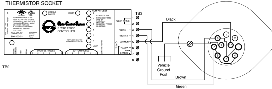
908-211 THERMISTOR SOCKET (Viewed from the rear)
