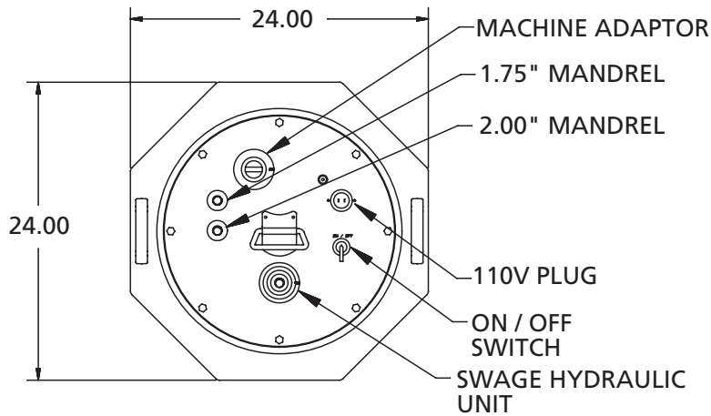
SWAGE KIT
