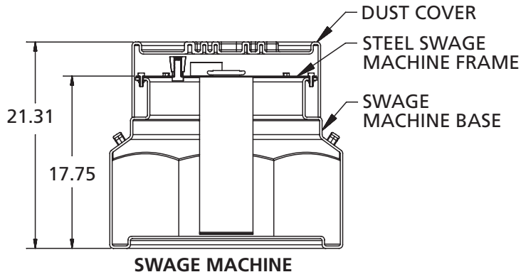
SWAGE MACHINE
