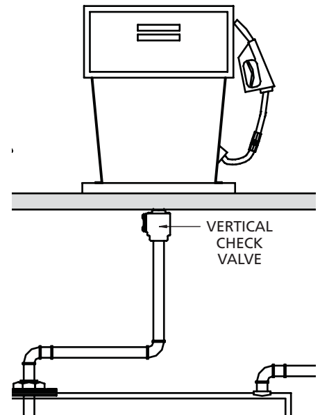
DOUBLE POPPET
