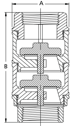
DOUBLE POPPET
