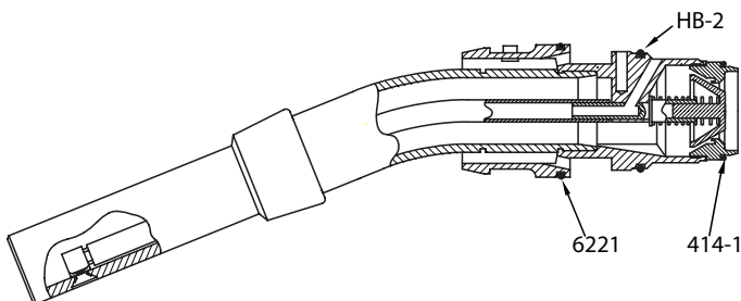
800 Series Spout O-Ring Locations
