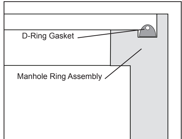
Figure 2: Gasket Orientation
