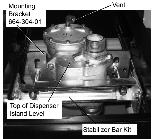
Figure 2: 644 Valve Installation
